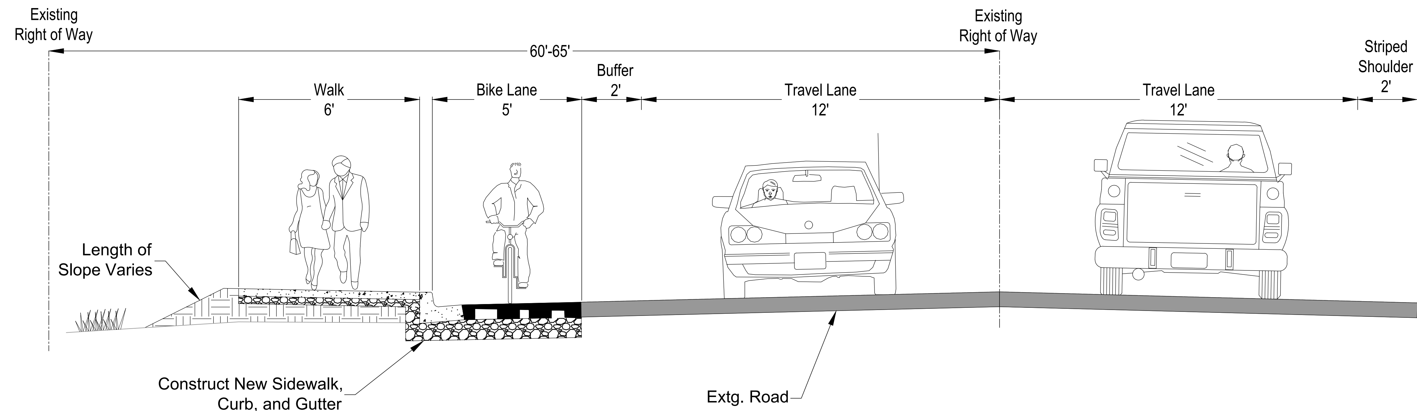
Cross Section: Terman Road Sidewalk
